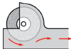
DIAGRAM 4 Good design carries away contaminants from the operator's breathing zone
