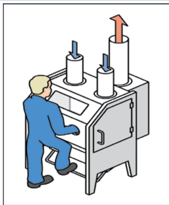
DIAGRAM 3 Enclosure around a grinding wheel
